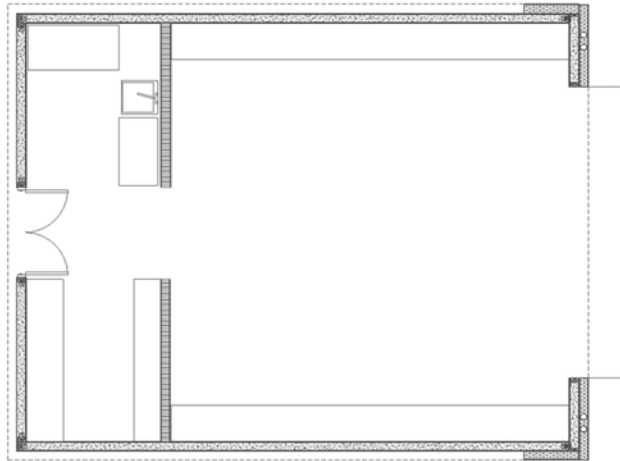
LVG FLOOR PLAN
